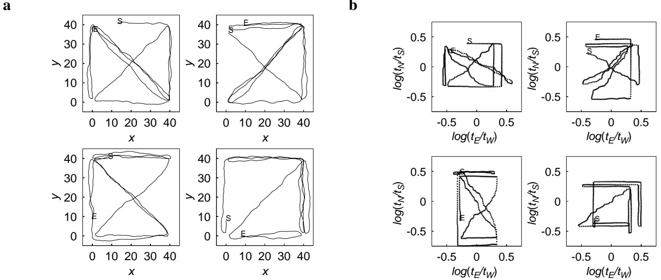
Figure 3. Physical space projects onto log firing rate space. A four-cell simulation with normalized inputs was run during simulated movements among the corners of a box. a. Successive paths of the simulated movement in physical space. b. The activity of the simulated neurons projected into log space for the sequences corresponding to a. The x axis in these plots is \log(t_E/t_W) , where t_E is the firing rate of the first unit, with preferred direction pointing toward the east. When the animal moves north/south, \log t_E/t_W is unchanged, despite the fact that both t_E and t_W are subject to exponential decay.
